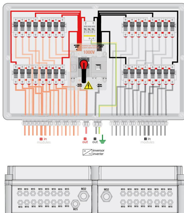
Model diagram 11...16 strings
